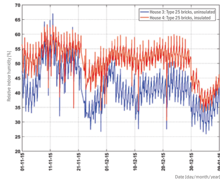
Comparing humidity in an insulated house - uninsulated house:
