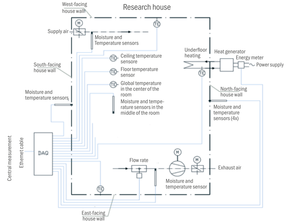
The measurement sensors in the research houses
